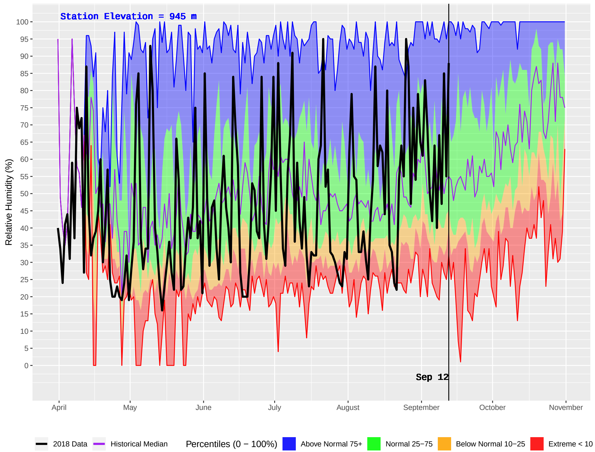
BOWRON HAGGEN (193) : Historical (1986–2016) and Current (2018) Daily Relative Humidity
